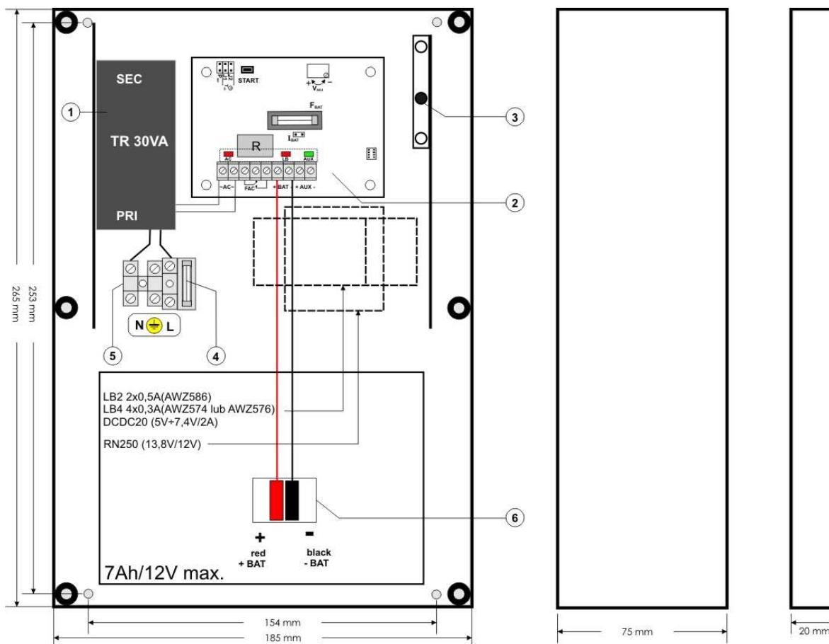
Fig.3. The view of the PSU.
