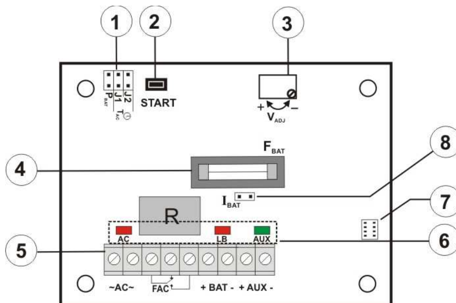
Fig.2. View of the pcb.
